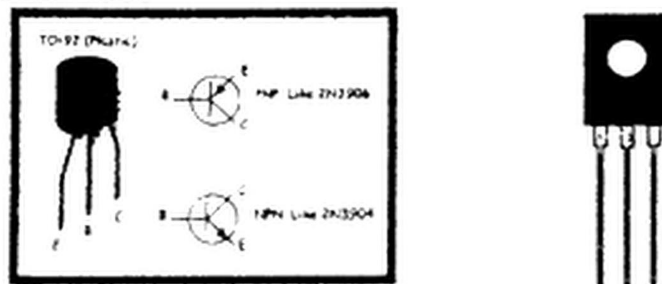
Transistor
